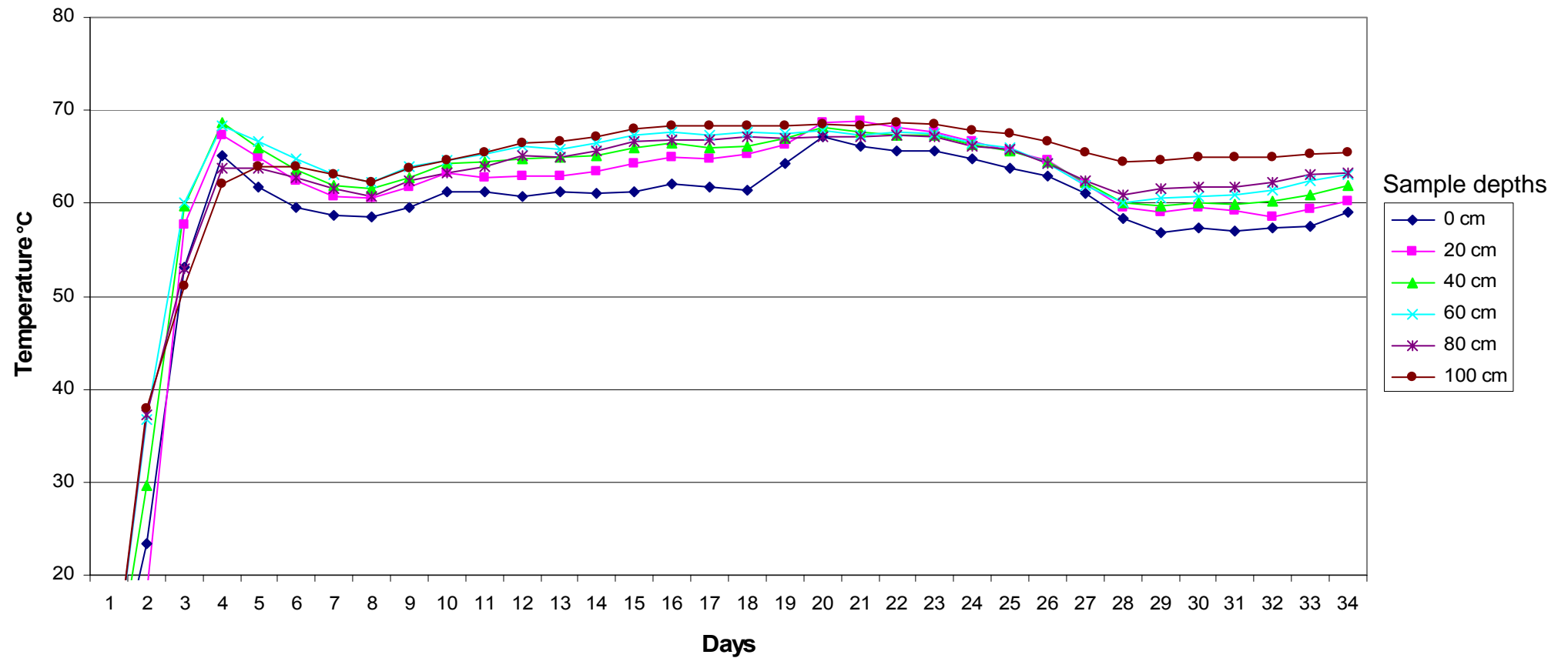
Typical Temperature-Time Correlation of Organic Composting Process with COMP-ANY System
